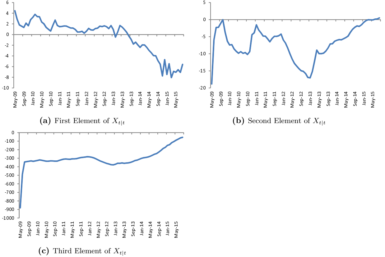
Figure 2: Time Series of Filtered Values X_{t|t}
